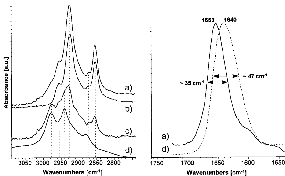
Figure 3. Analysis of the CH-stretching region ( 3000\text{--}2800\text{ cm}^{-1} ) and the amide I band around 1650\text{ cm}^{-1} . (a) ER FTIR spectrum of PPEI grown on the triflate functionalized HUT SAM. (b) ER FTIR spectrum of HUT SAM. (c) Subtraction result of (a)–(b). (d) Bulk spectrum of PPEI.
